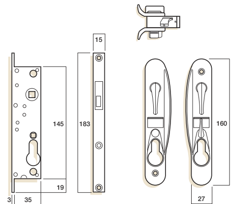
Cylinder locking
